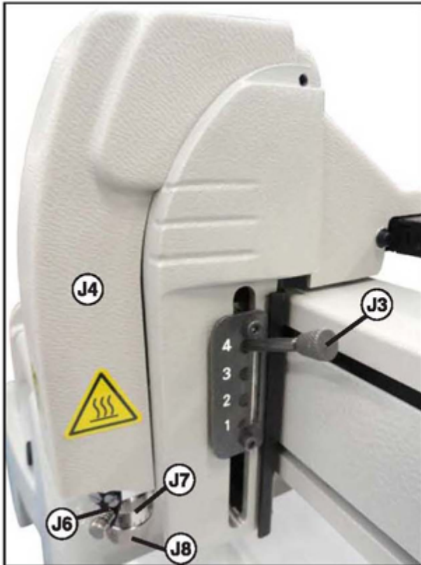
Tool holder
