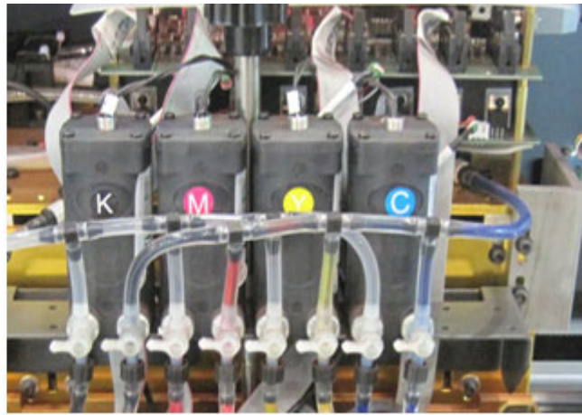
Ink Supply and Nozzle Cleaning System
