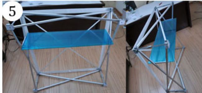
5. Place the board.
