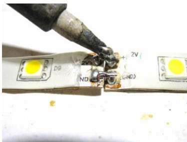
Solder Connection
