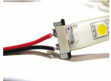
Splice Connector
