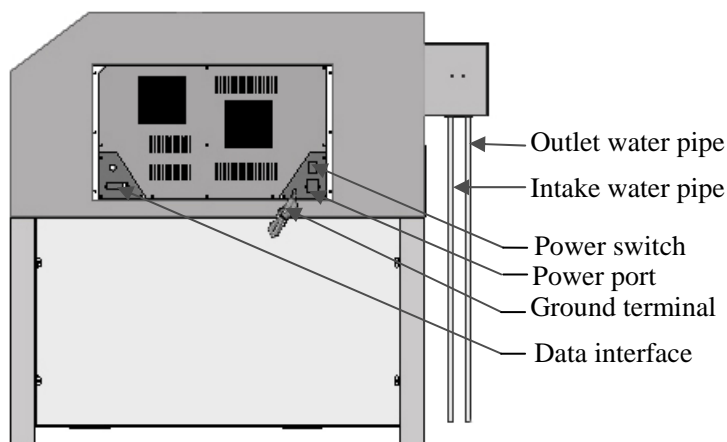
Pic.2-5 Right side of the machine
