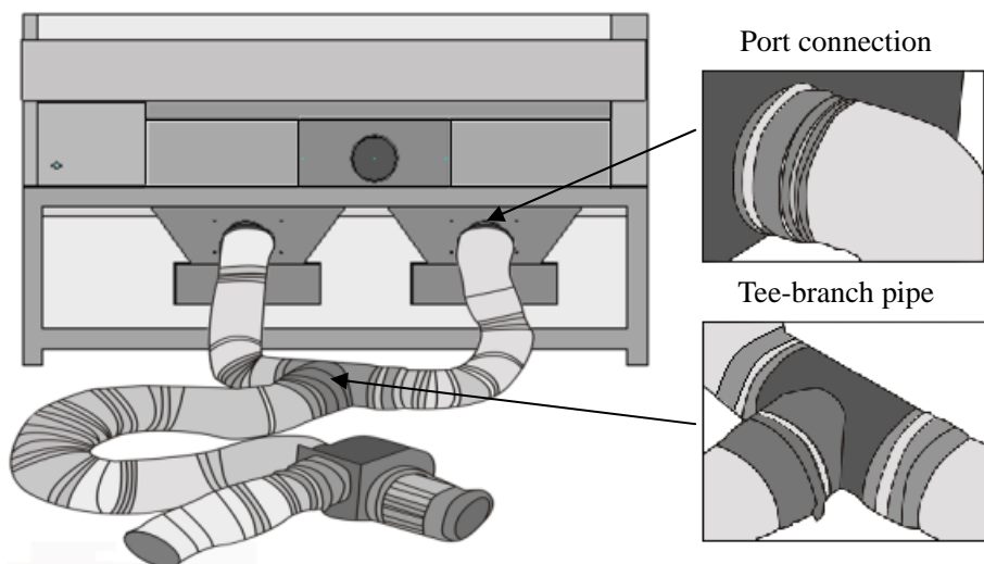
Pic2-9 downward air exhaust system
