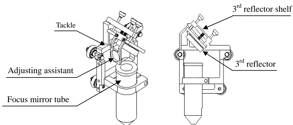
Pic.2-13 Laser head configuration
