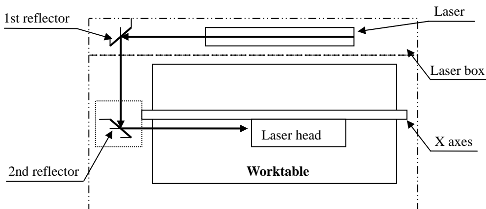
Pic.2-12 Optical path
