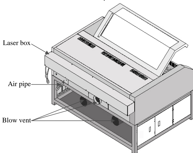
Pic.1-2 Rear of the machine
