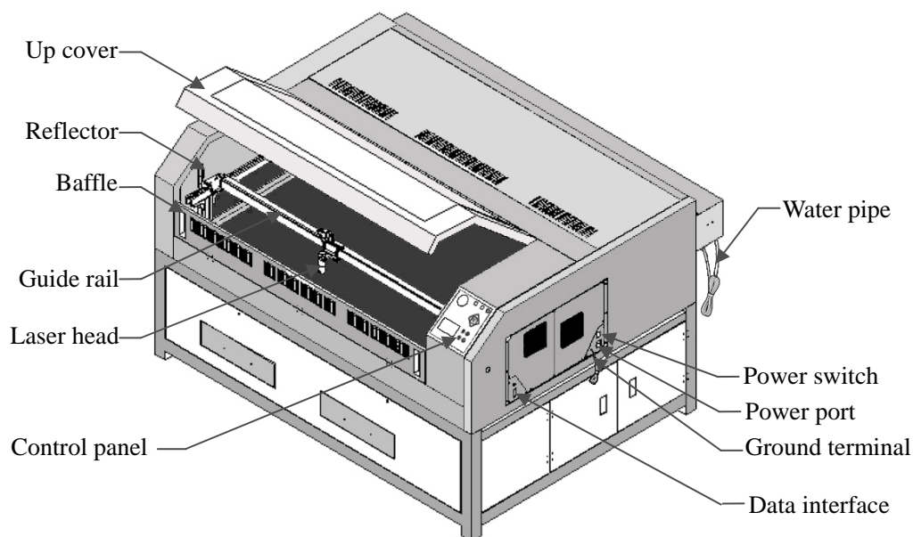
Pic.1-1 Frontispiece of the machine
