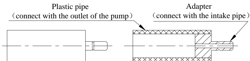
Pic.2-6 Adapter
